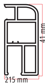
FCTD - 41 413gr/m folha mosquito deco iTEC | euroTECplus
